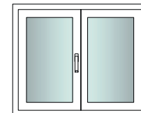
MH-DF Madriers: 15mm Dim.: 110x92cm
