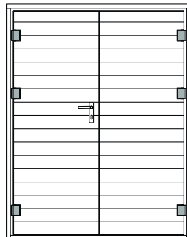
MH-DT-GG-WB Madriers: 15mm Dim.: 150x194cm
